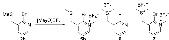
Scheme 3. Product mixtures obtained upon alkylation of 2b .
